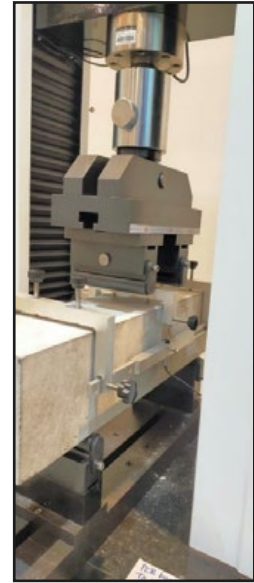
ASTM C1609 Setup
